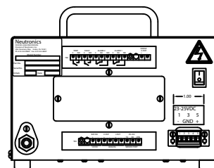
Back view - 24 VDC
